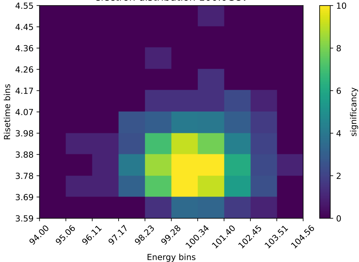
electron distribution 100.0GeV
